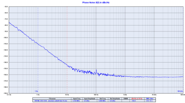
TWTMC-EXO 6.144 MHz phase noise
